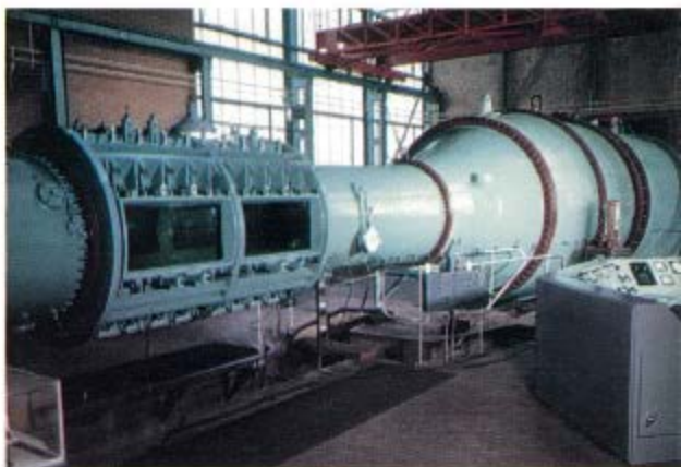
Close-up of Water Tunnel test section. Note narrowing chamber, viewing section and dogging down gear. Instrumentation is at right.
