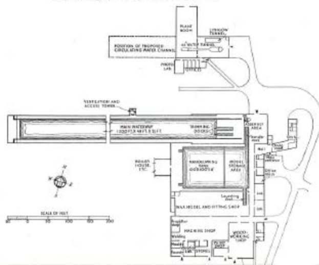
House of the Ship Hydrodynamics Laboratory at Feltham with small map showing location of the various facilities.
