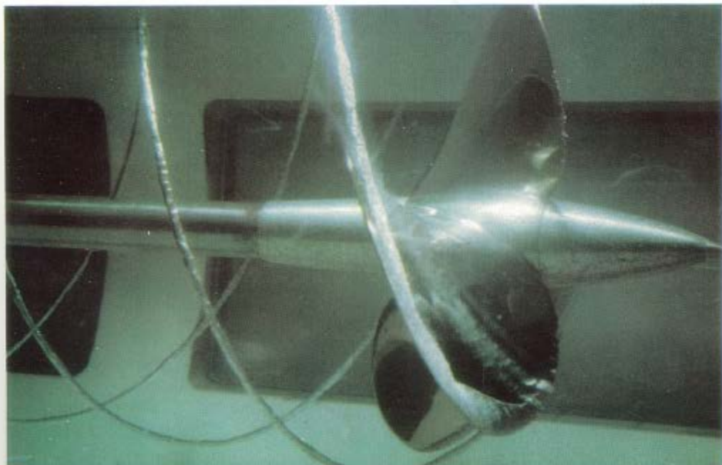
Striking photograph of a propeller model under test clearly showing cavitation.
